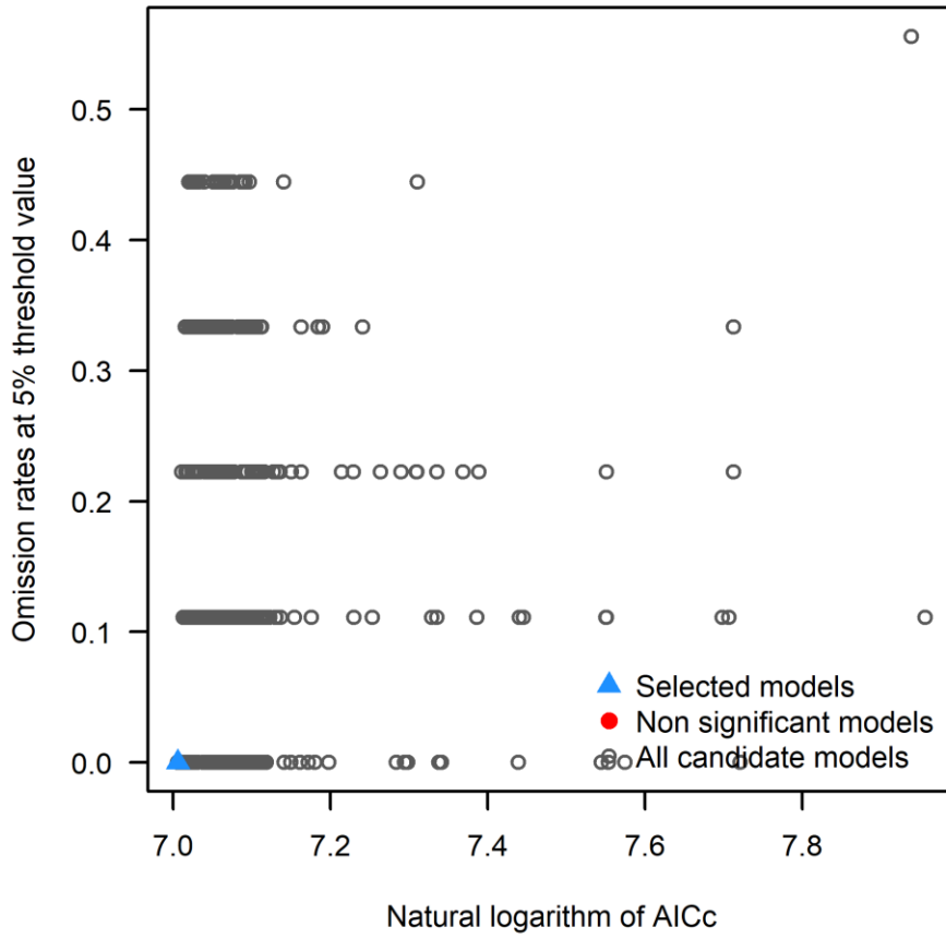
2 3 Supplementary Figure 1. Omission rates and natural logarithm of AICc for every model 4 evaluated, selected model is indicated by a blue triangle having the lowest values. 5 6
